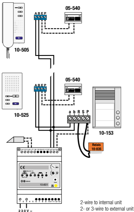
fig.1: complete connection diagram
