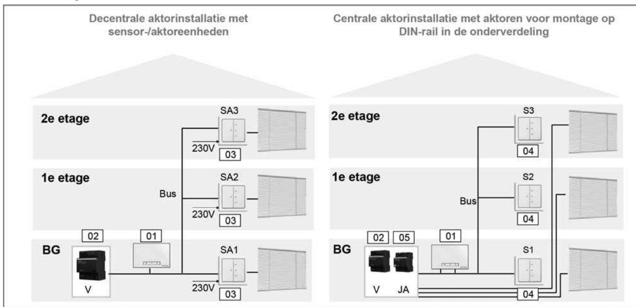
Afb. 2 Planning actoren
